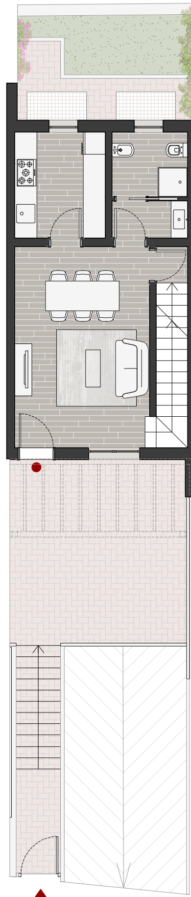
Piano terra
