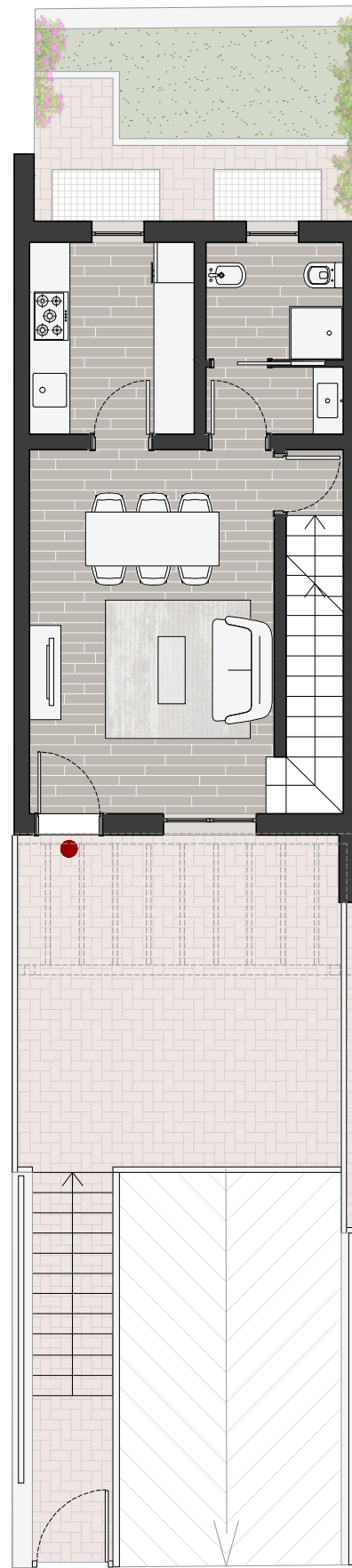
Piano terra
